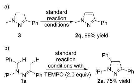
Scheme 2. Control experiments. TEMPO = 2,2,6,6-tetramethylpiperidin-1-oxyl.
