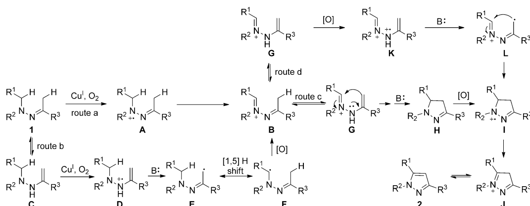
Scheme 1. Plausible reaction mechanism.
